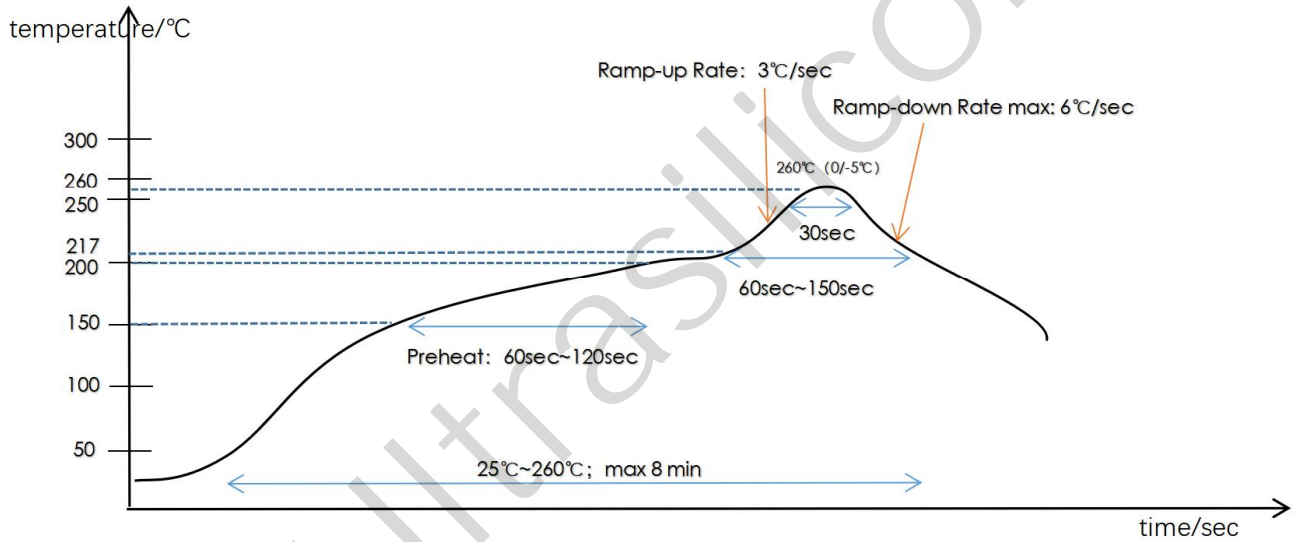
Figure24: Recommended Temperature(PB-Free)
